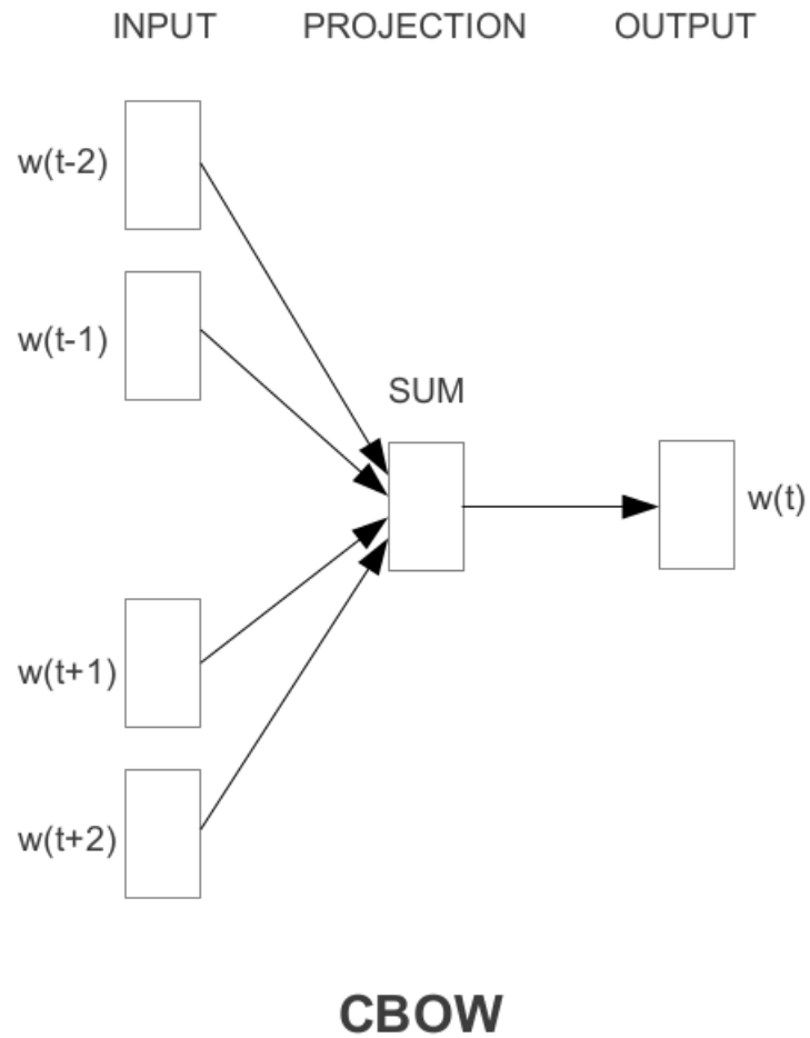
Figura 17: CBow architecture
